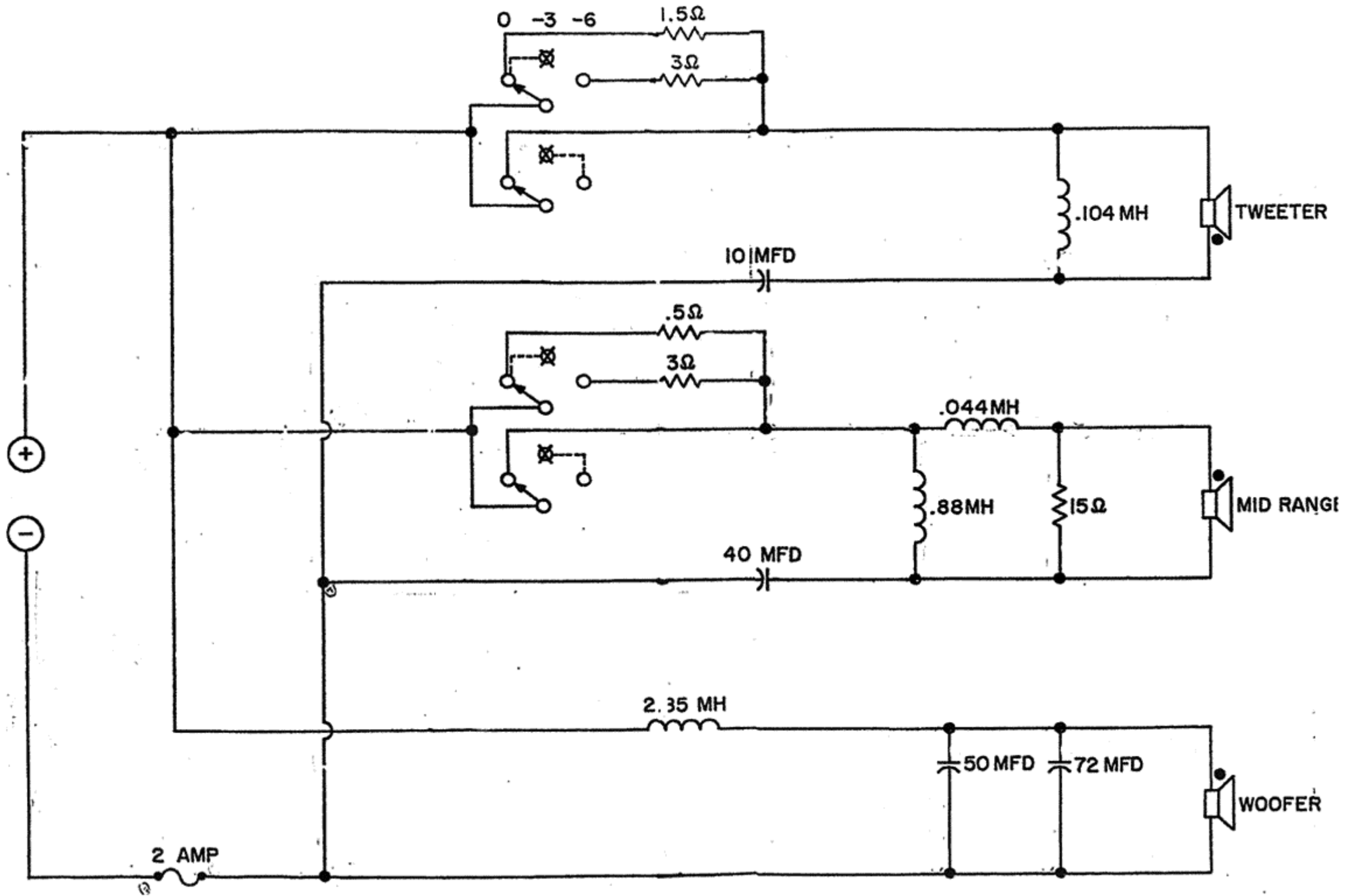
AR-II SCHEMATIC
