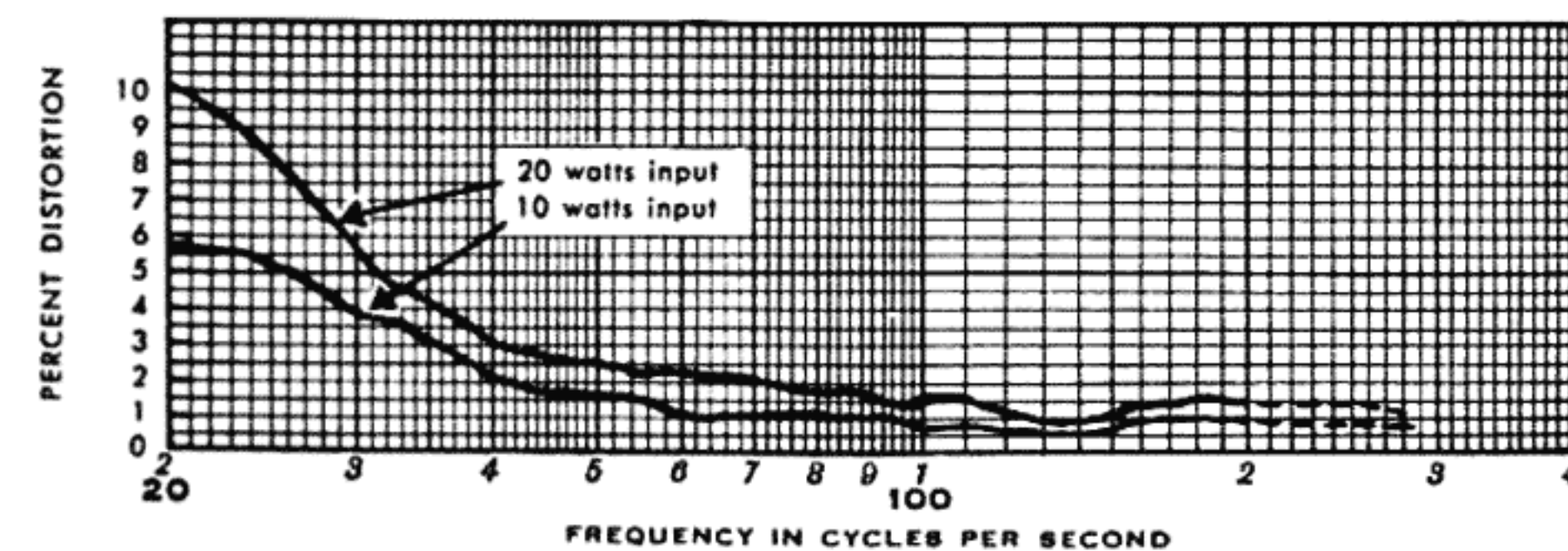
Figure 4: Low-Frequency Distortion
