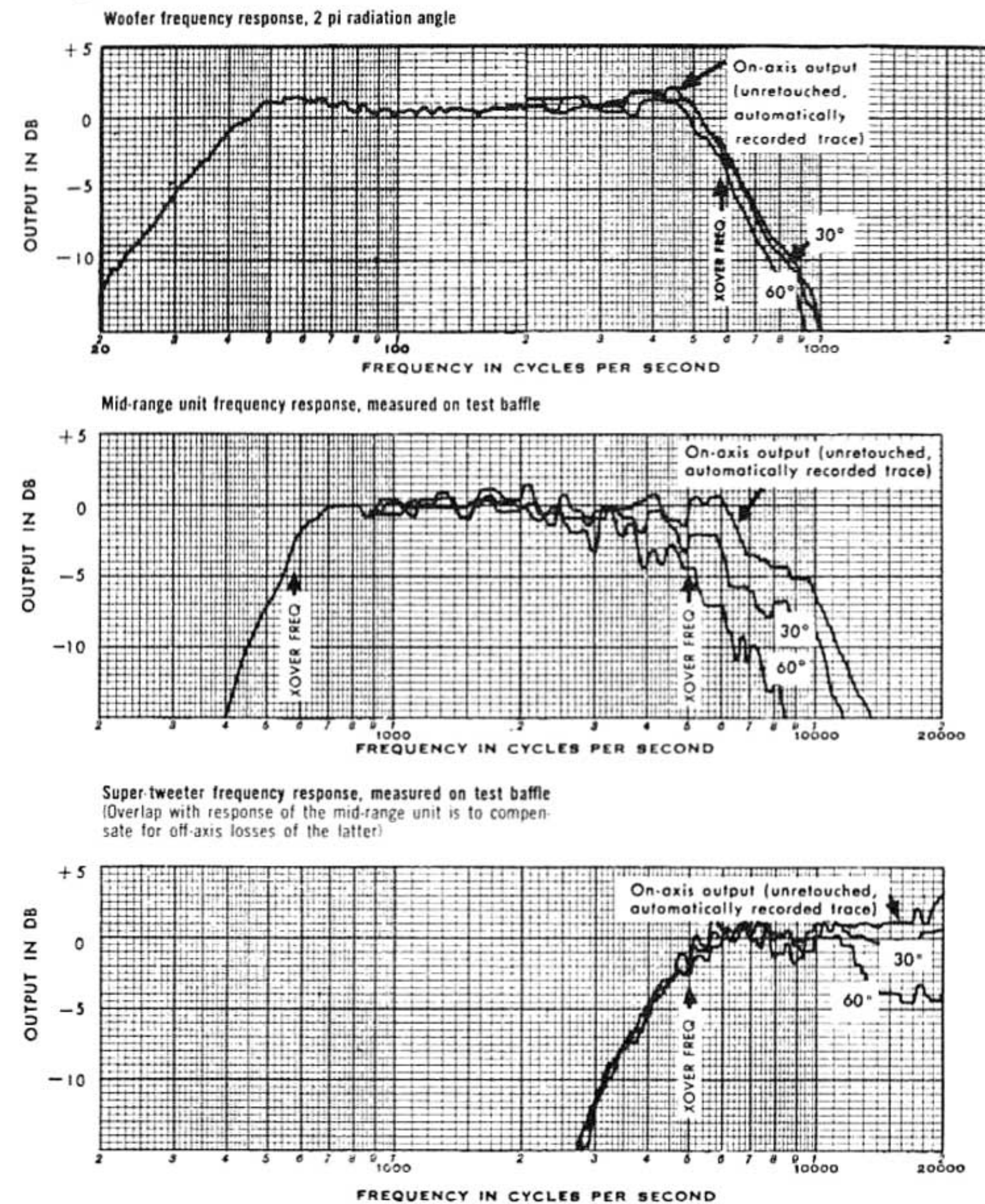
Figure 3: Anechoic Response of Individual Drivers
