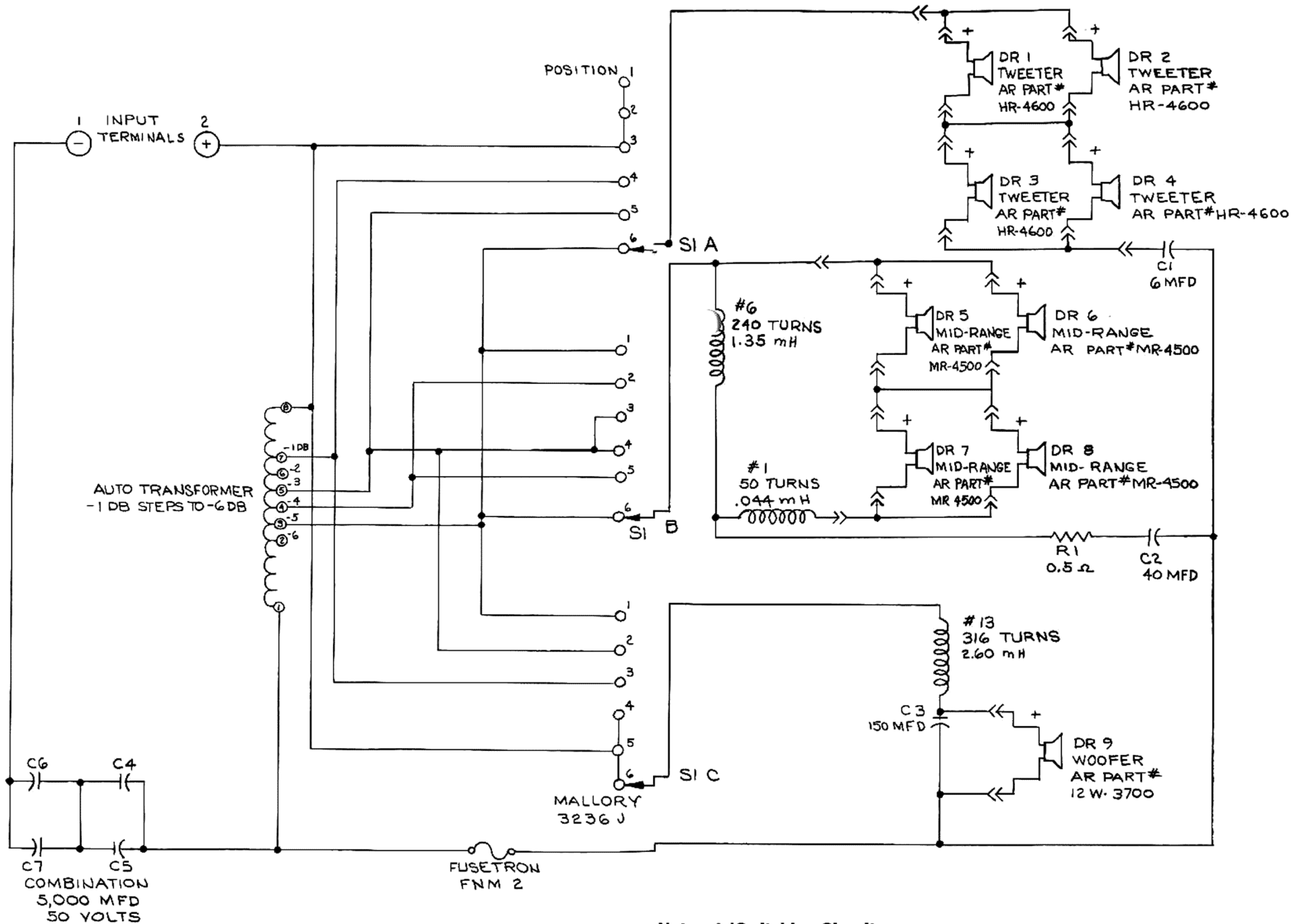
Figure 5: AR-LST Crossover Network/Switching Circuit
