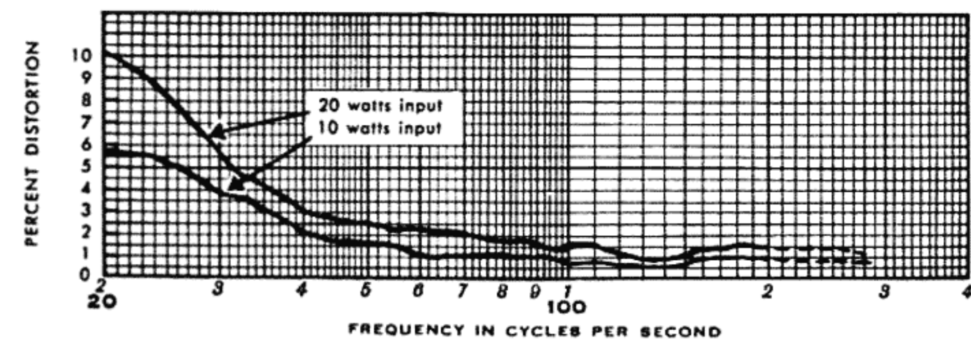
Figure 4: Low-Frequency Distortion
