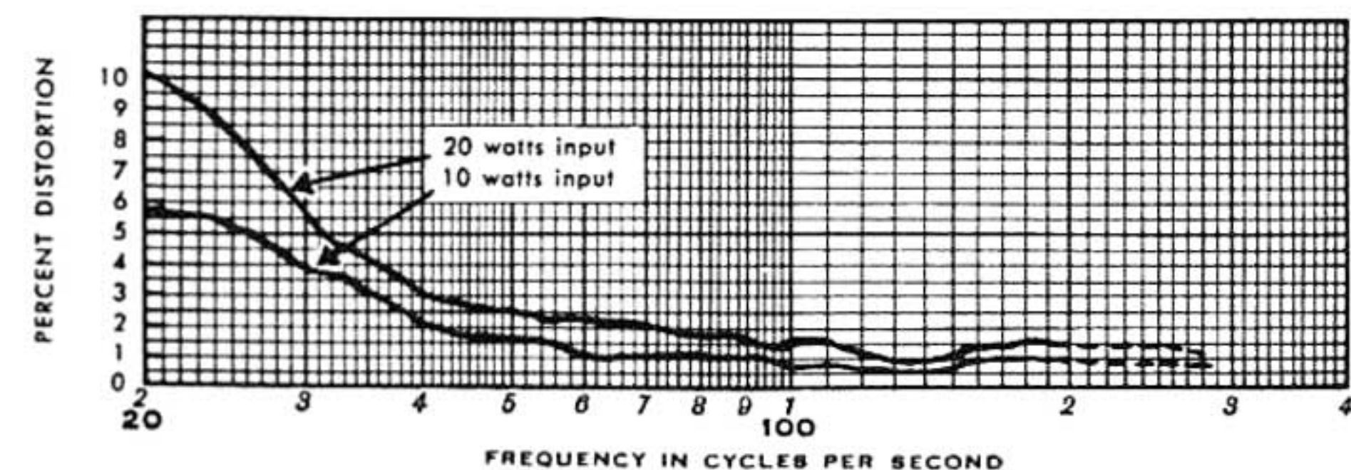
Figure 4: Low-Frequency Distortion
