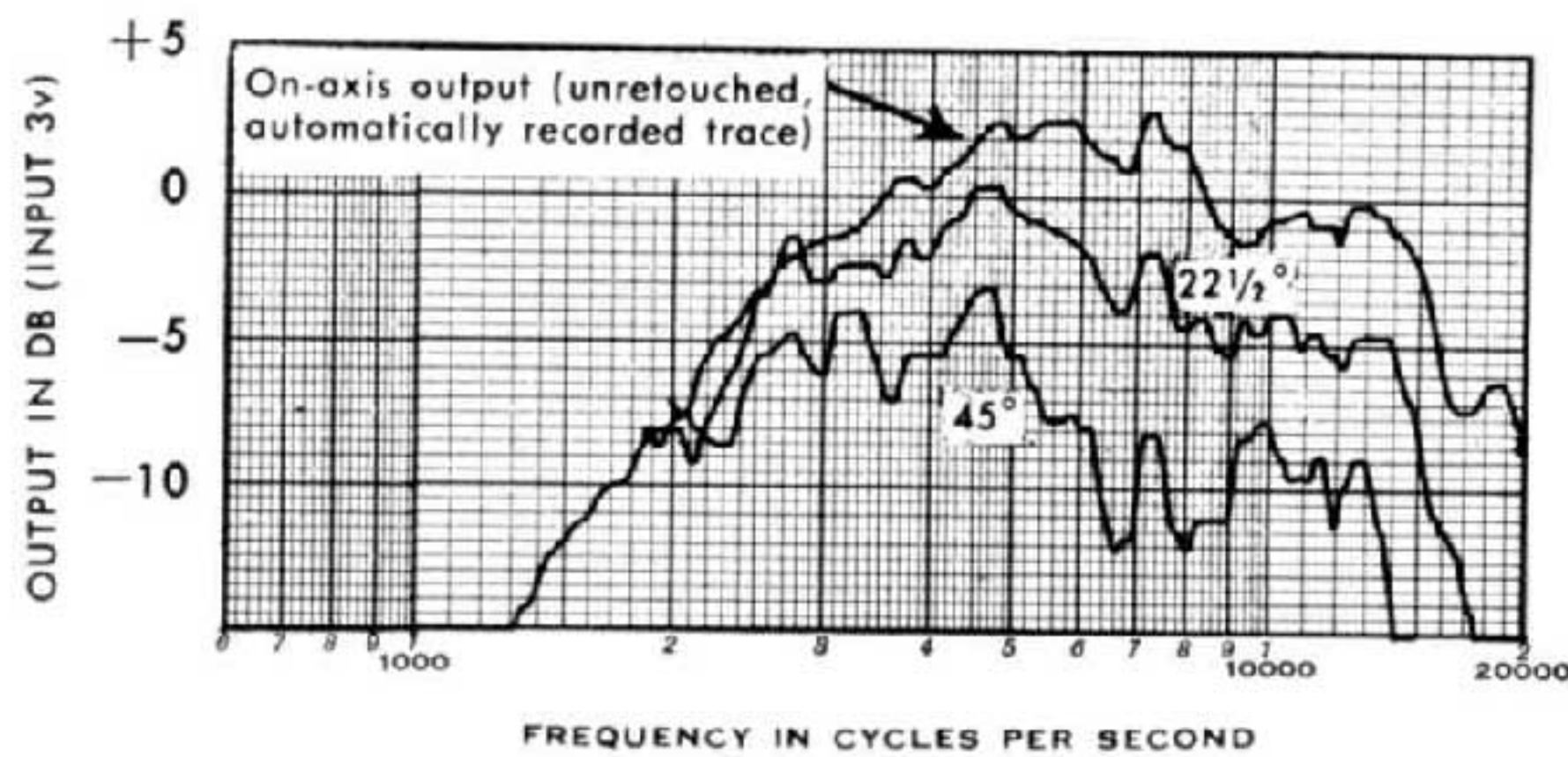
AR-2 tweeter (AR-2a mid-range) frequency response—single speaker in test baffle Two of these tweeters are used, each radiating 20° off-axis in opposite directions.
