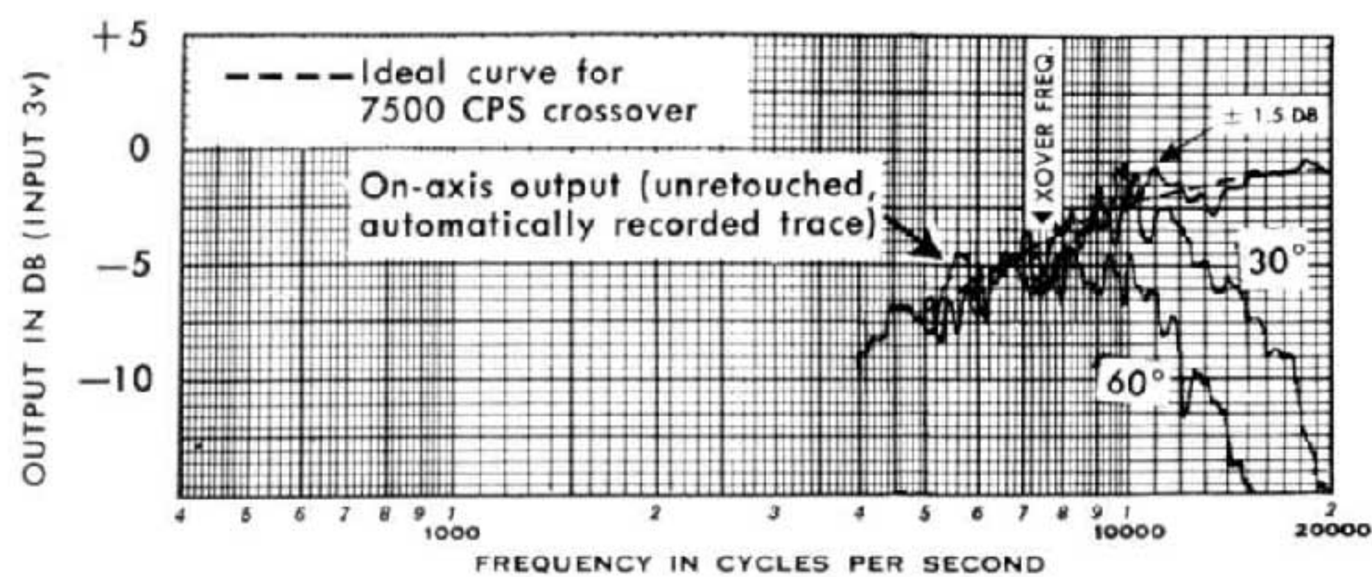
AR-2a super-tweeter frequency response
