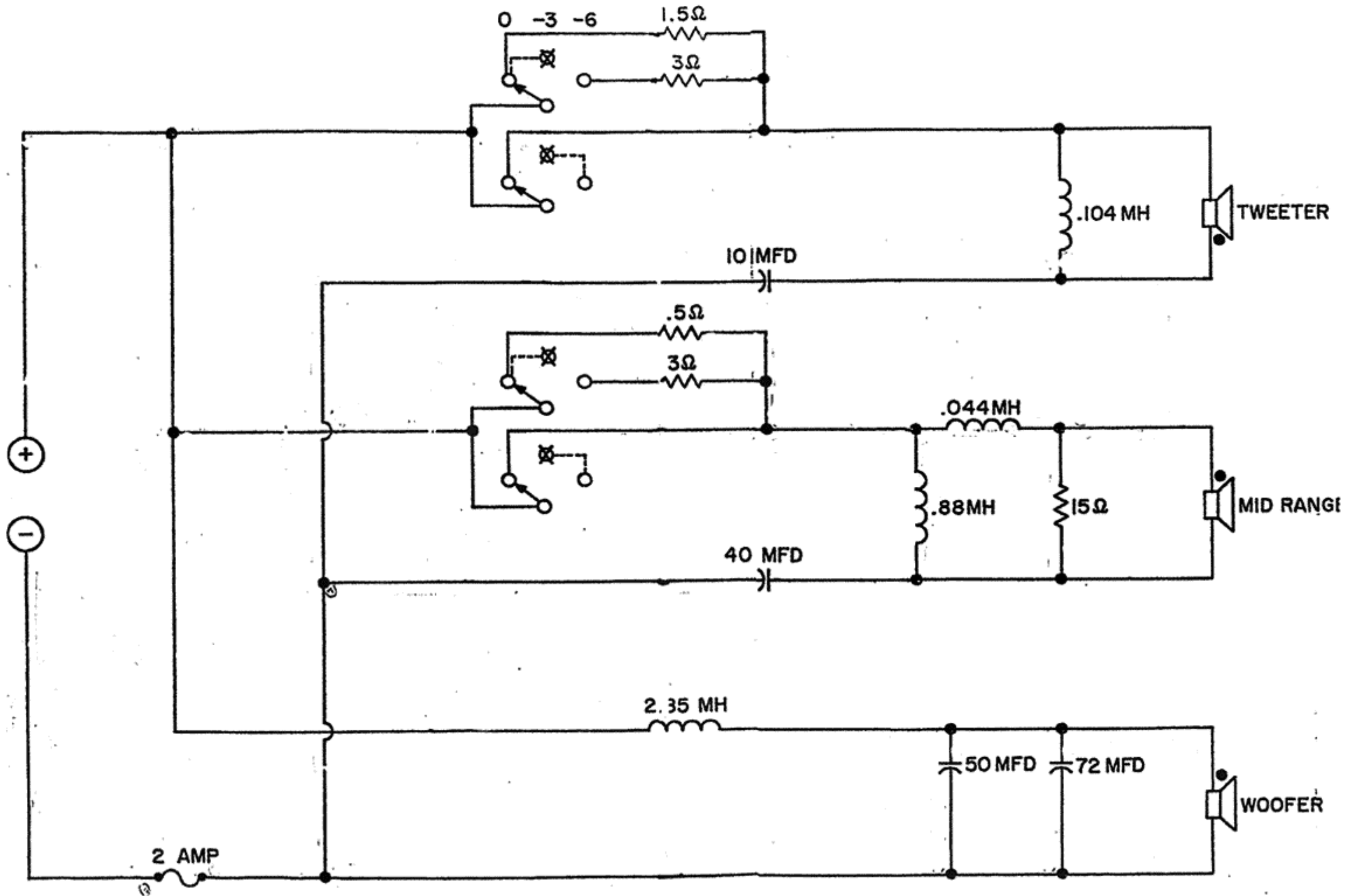
AR-II SCHEMATIC
