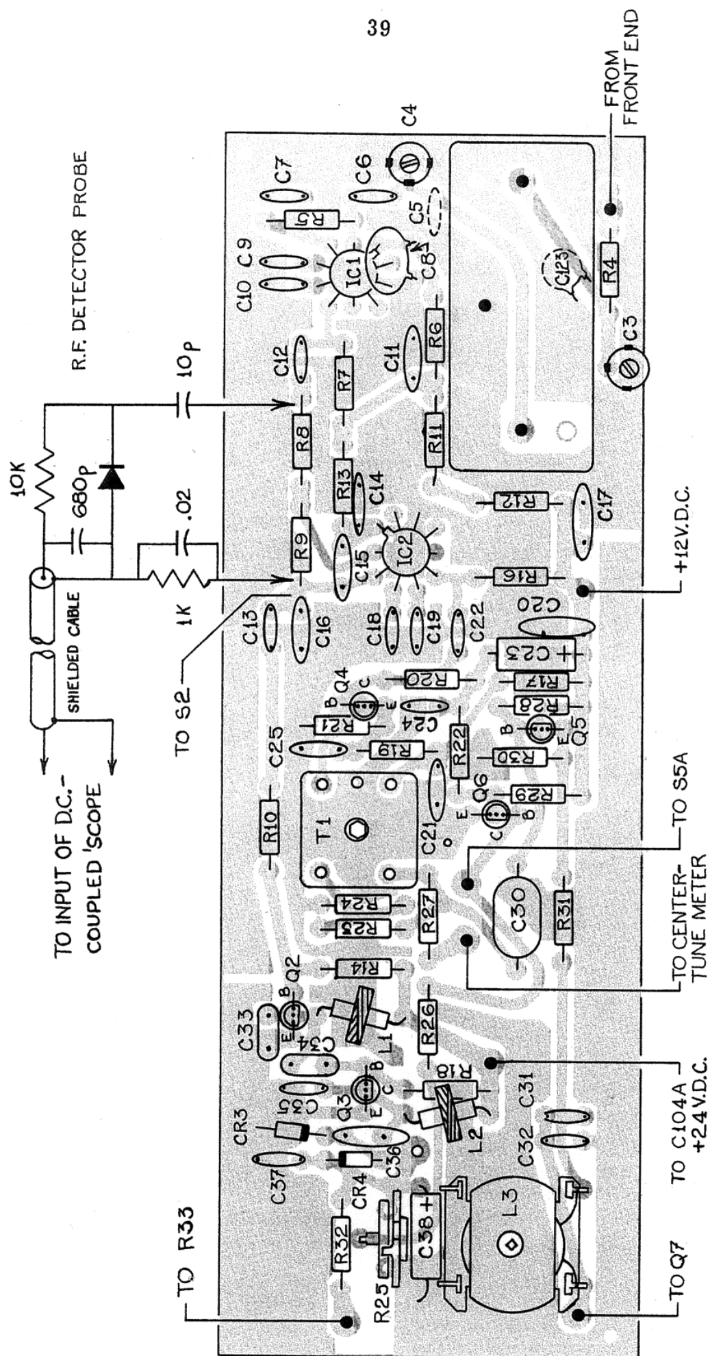
FIGURE 13 IF BOARD
