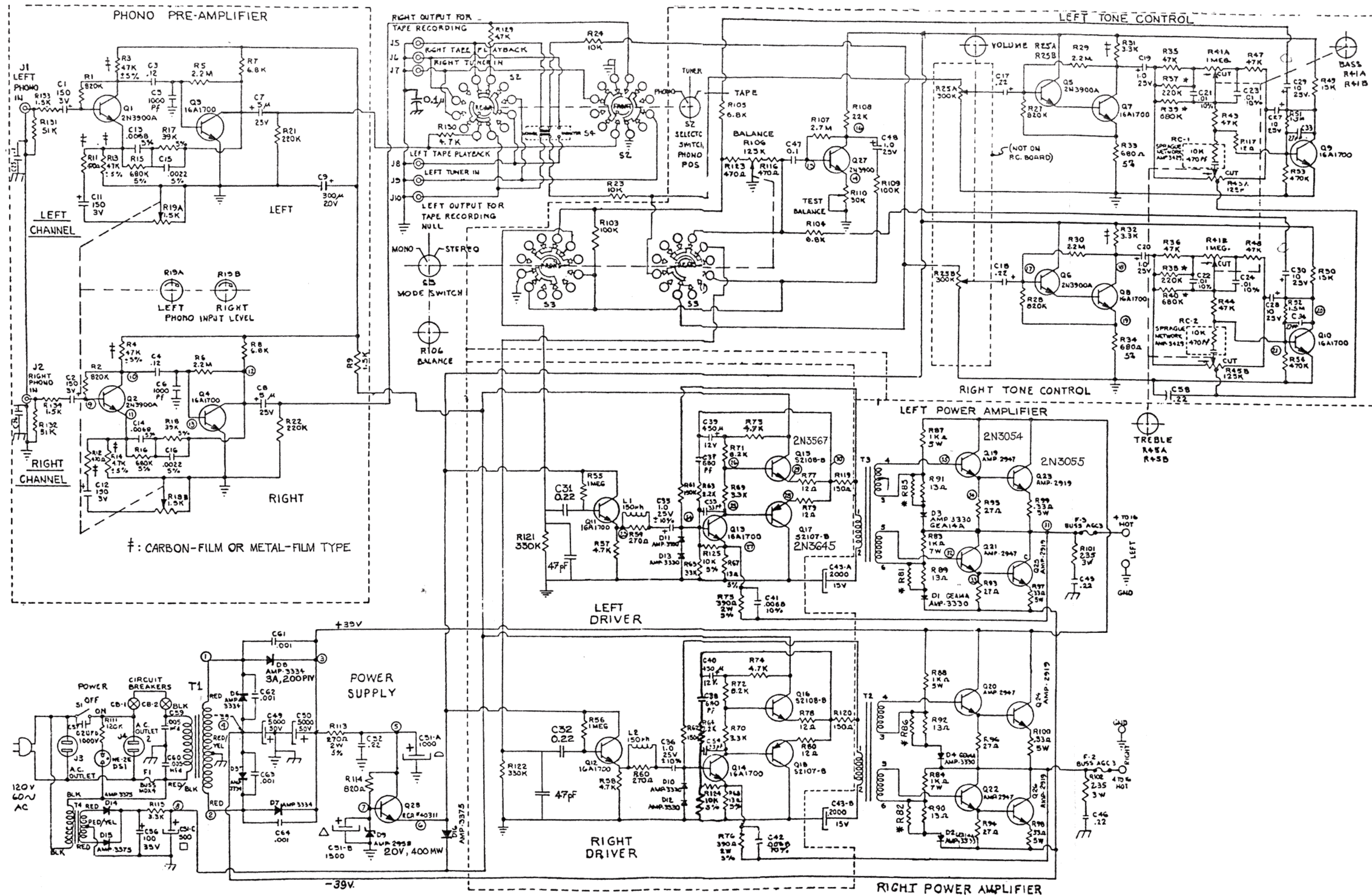
FIGURE 1 AMPLIFIER SCHEMATIC
