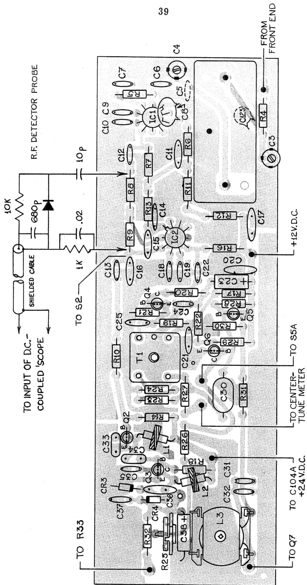
FIGURE 13 IF BOARD
