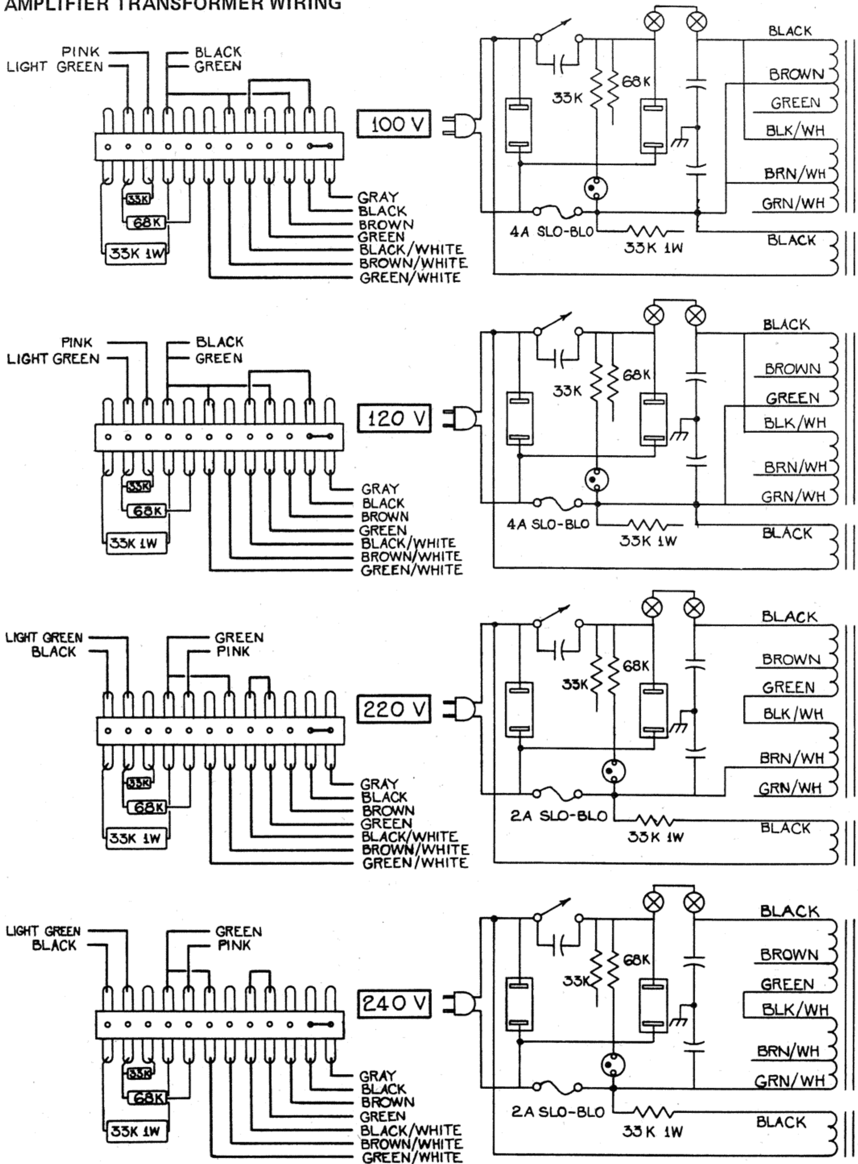
FIGURE 16 AMPLIFIER TRANSFORMER WIRING
