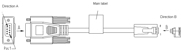
Figure 102 Console cable
